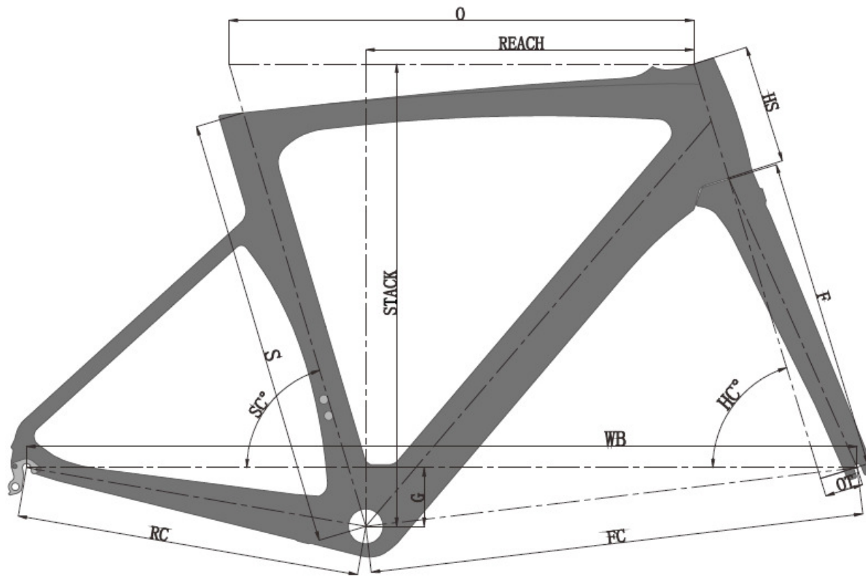
Aero-race 19 Length in mm
